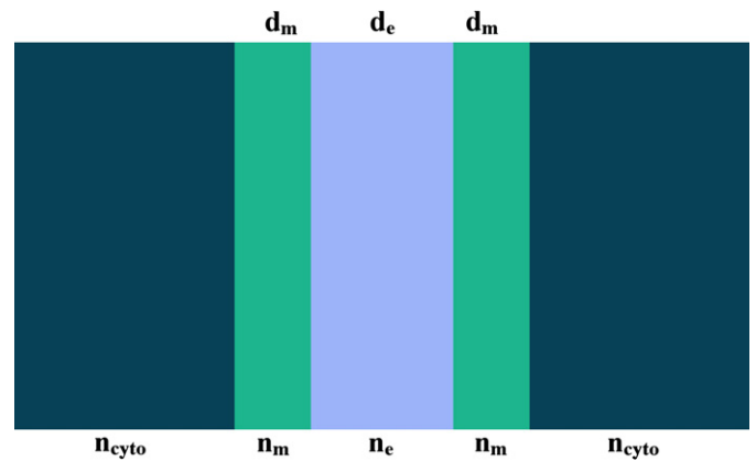
Fig. 3. Schematic of the layers at nuclear fiber cell interfaces. The dimensions of each membrane, d_m , is 7 nm and of the ECS, d_e , is variable from 1 nm to 100 nm. As described in the text, the refractive index of the cytoplasm, n_{\text{cyto}} , is between 1.40 and 1.42, of the membranes, n_m , is higher at about 1.50 and of the ECS, n_e , is lower at about 1.35. These values can be varied to reflect aging and cataract formation.
