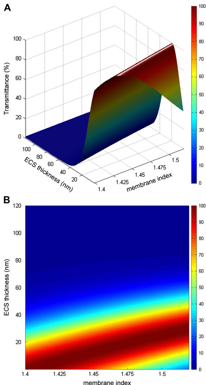
Fig. 10. Theoretical calculation of the percent transmittance for a nucleus containing 4000 membrane interfaces with layers as described in Fig. 3. (A) Surface plot for n_{\text{cyto}} = 1.42 and n_e = 1.35 . Nearly 100% transmittance is predicted for ECS thicknesses of 15–20 nm for n_m = 1.50 . (B) Flat projection view for the same conditions in A except for n_{\text{cyto}} = 1.40 . Note that the 100% transmittance at n_m = 1.50 occurs at about 25–30 nm and that there is a very steep drop in transmittance above 35 nm.
